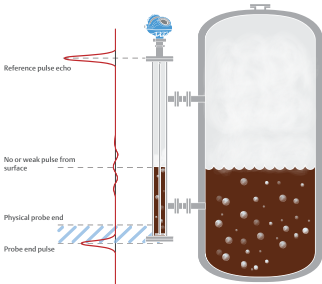
With Probe End Projection, the surface position is calculated when the surface echo is unavailable
