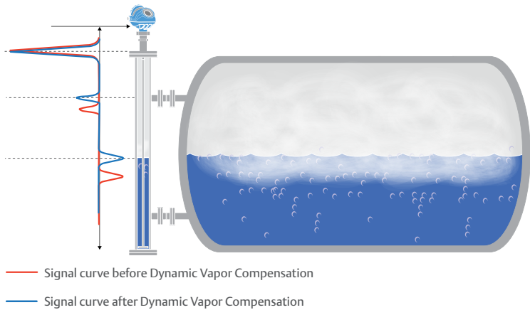
The steam dielectric is measured by using a vapor probe with a reference reflector
