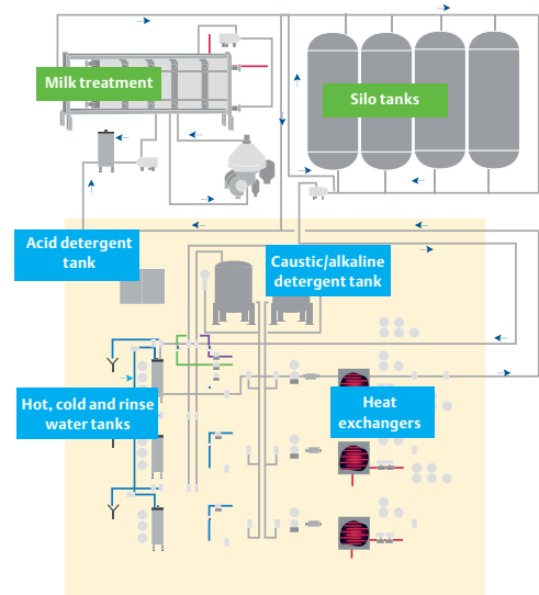
Principle of a centralized CIP system
