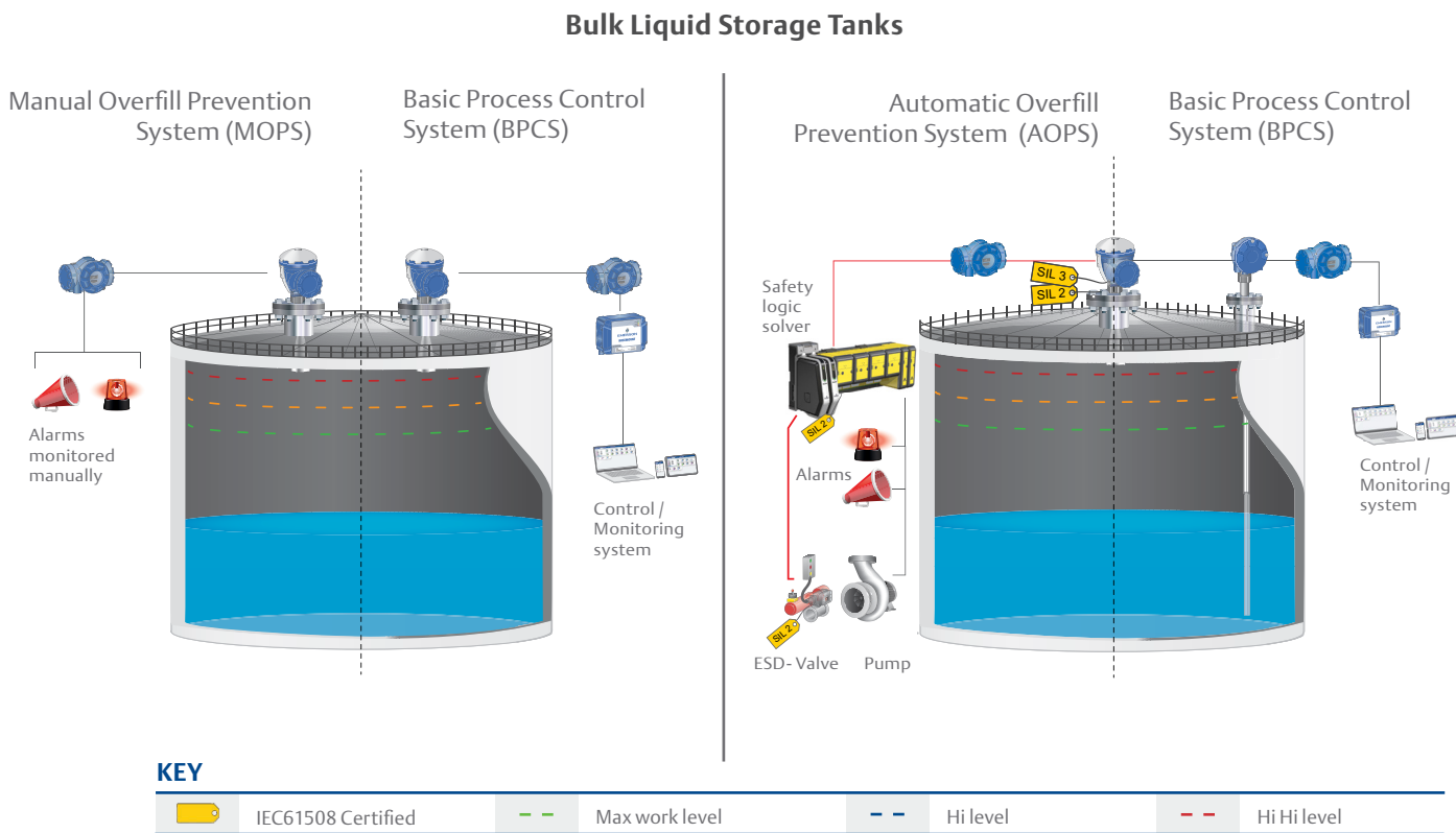
Level sensors for bulk liquid storage overfill prevention
