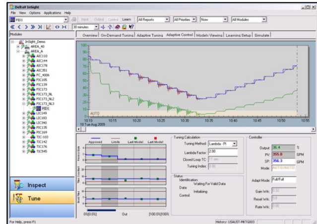
DeltaV Adaptive Control
