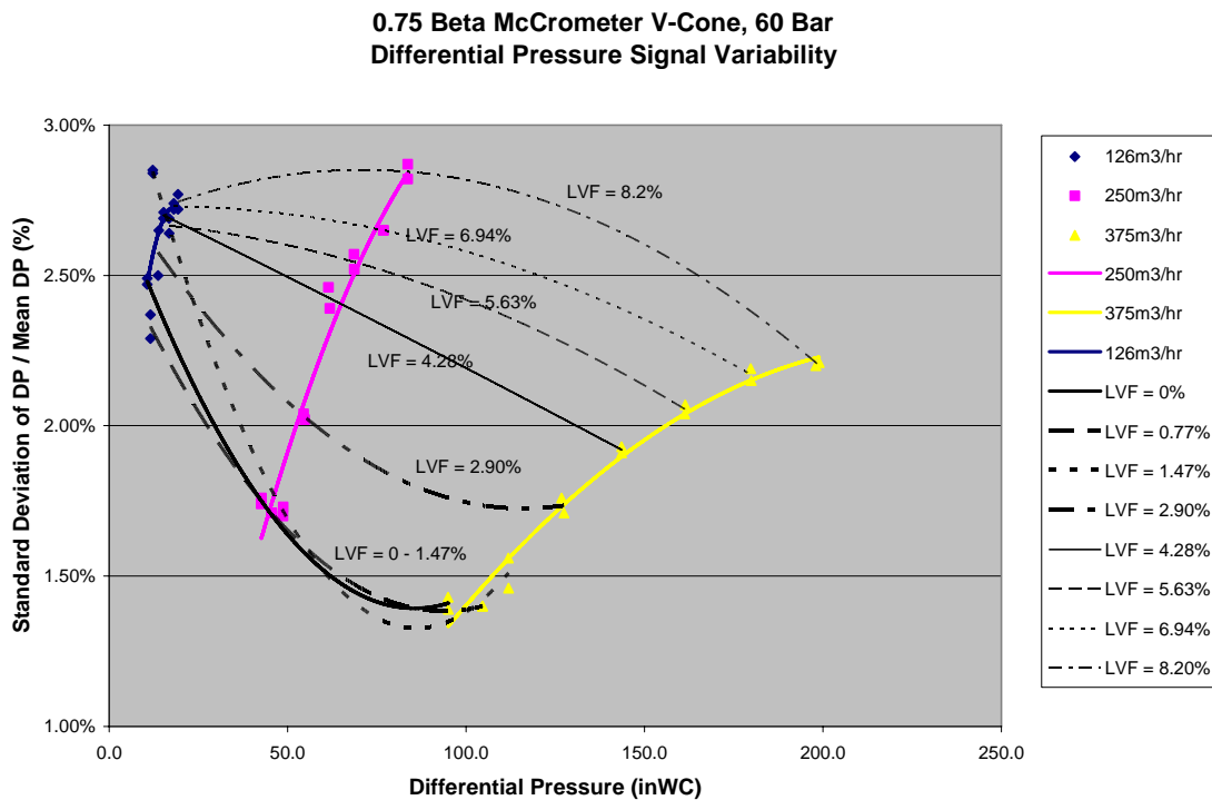
Figure 11: DP signal variability for 0.75 beta McCrometer V-Cone at 60 bar
