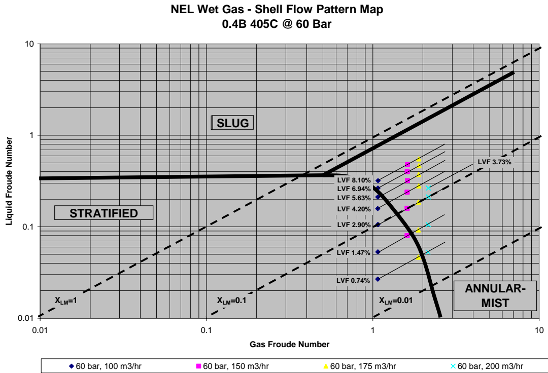
Figure 6: Shell Flow Pattern Map for 0.4 beta Rosemount 405C compact orifice plate at 60 bar
