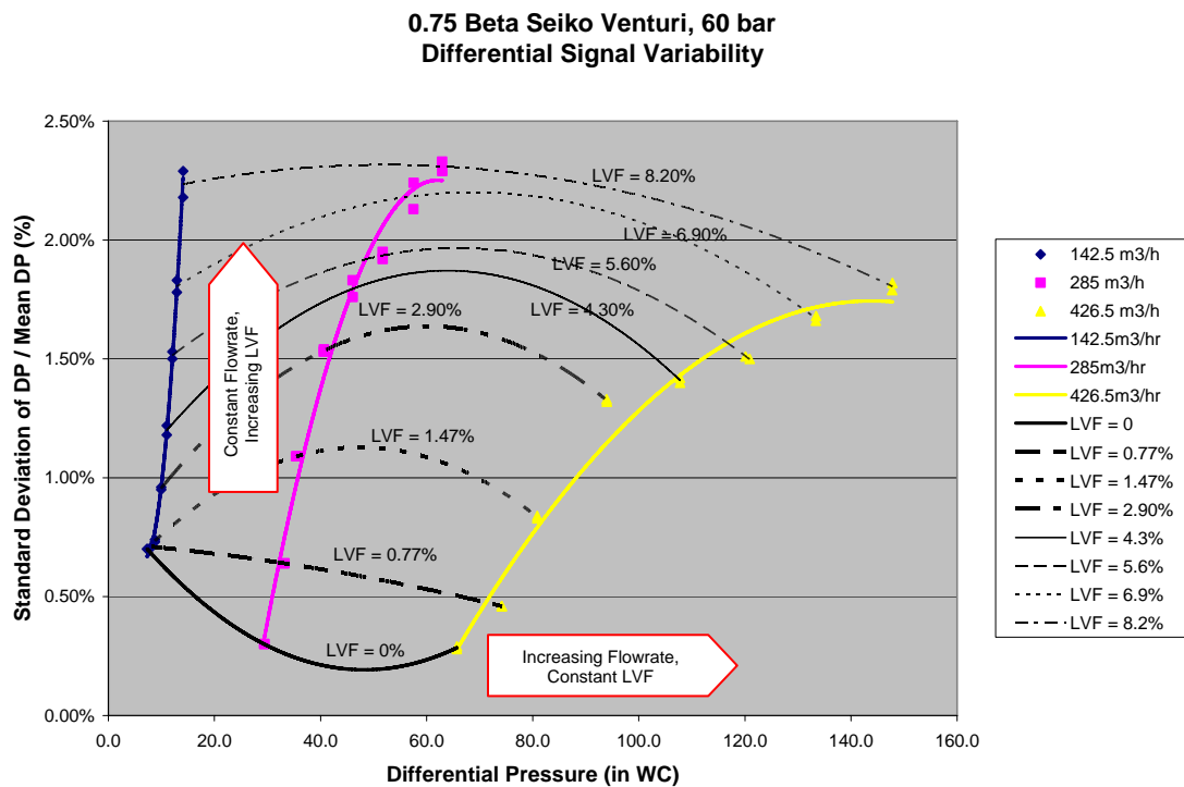
Figure 5: DP signal variability for 0.75 beta Seiko Venturi at 60 bar
