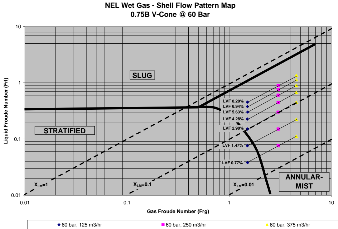
Figure 10: Shell Flow Pattern Map for 0.75 beta McCrometer V-Cone at 60 bar
