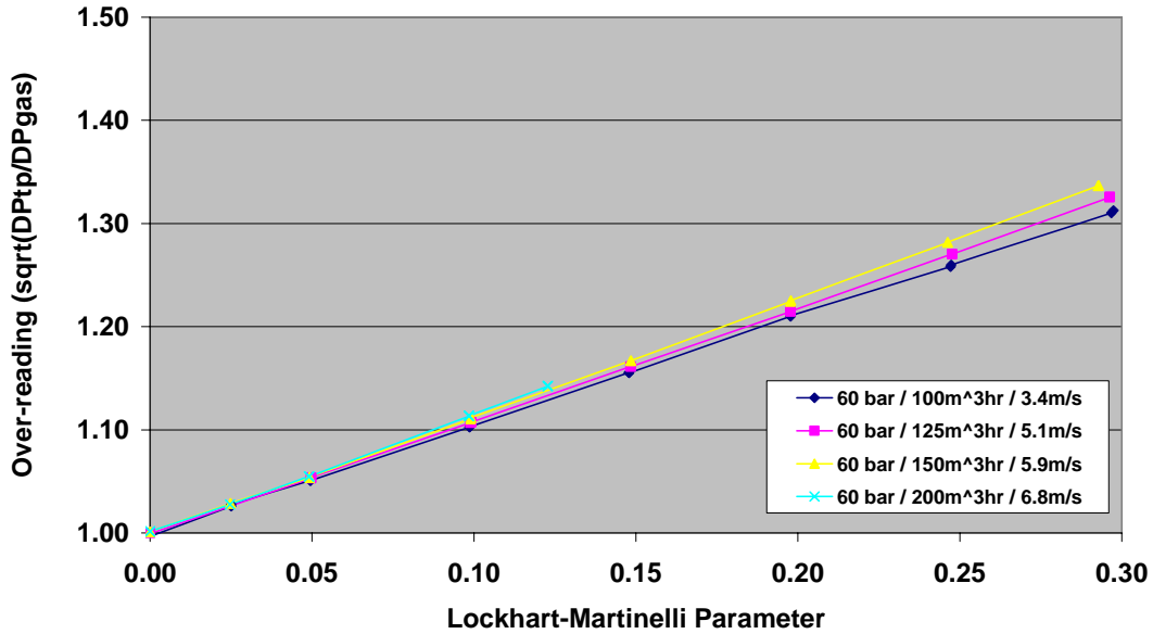
Figure 2: Relationship between Lockhart-Martinelli parameter and overreading for a Compact Orifice Plate
