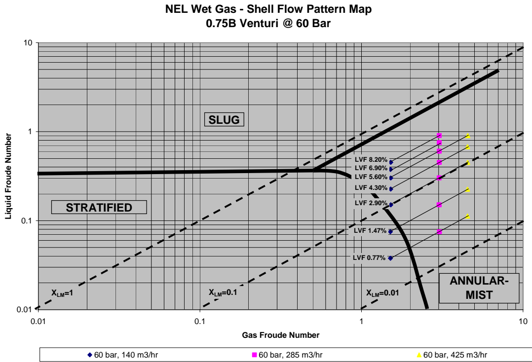
Figure 4: Shell Flow Pattern Map for 0.75 beta Seiko Venturi at 60 bar
