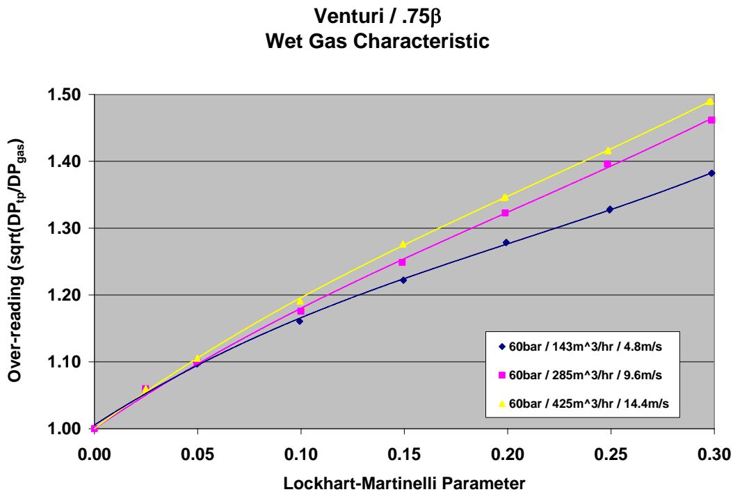
Figure 1: Relationship between Lockhart-Martinelli parameter and overreading for a typical Venturi
