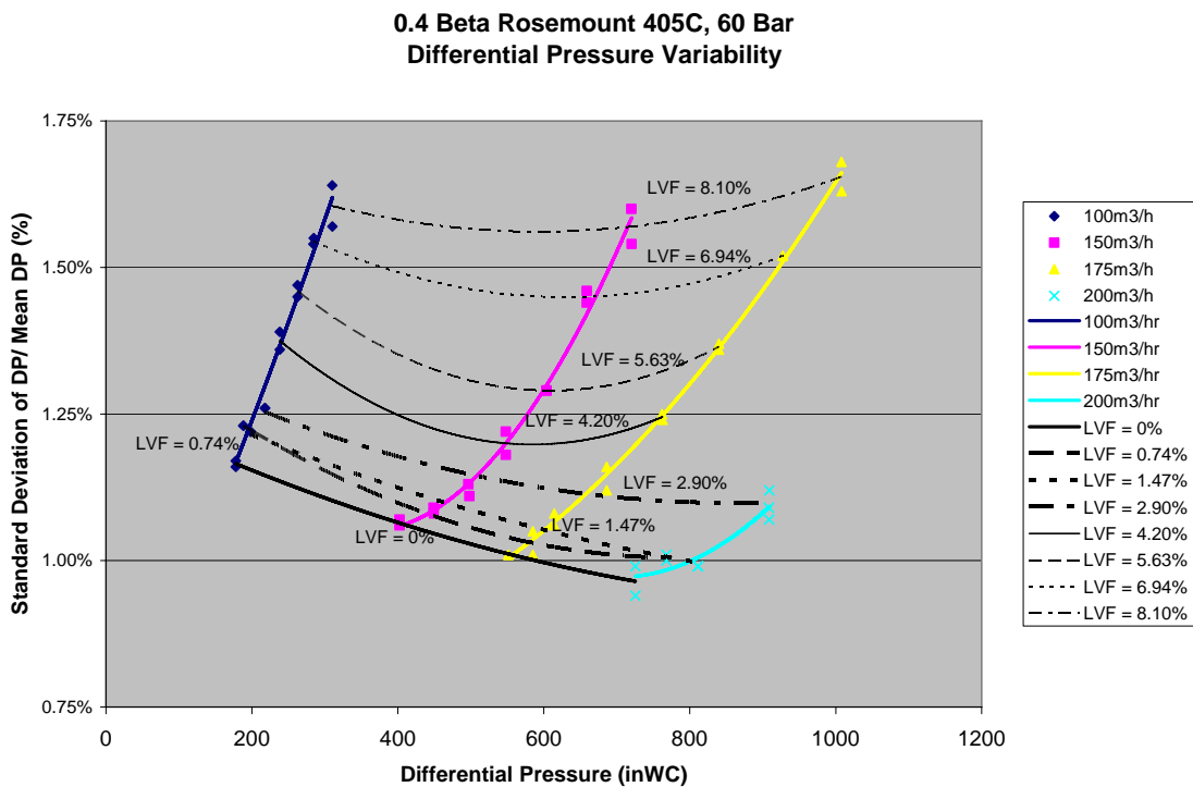
Figure 7: DP signal variability for 0.4 beta Rosemount 405C compact orifice plate at 60 bar
