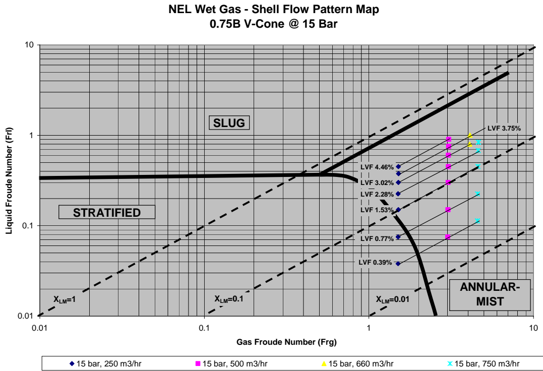
Figure 8: Shell Flow Pattern Map for 0.75 beta McCrometer V-Cone at 15 bar
