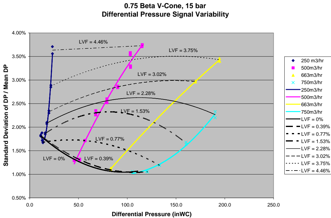
Figure 9: DP signal variability for 0.75 beta McCrometer V-Cone at 15 bar
