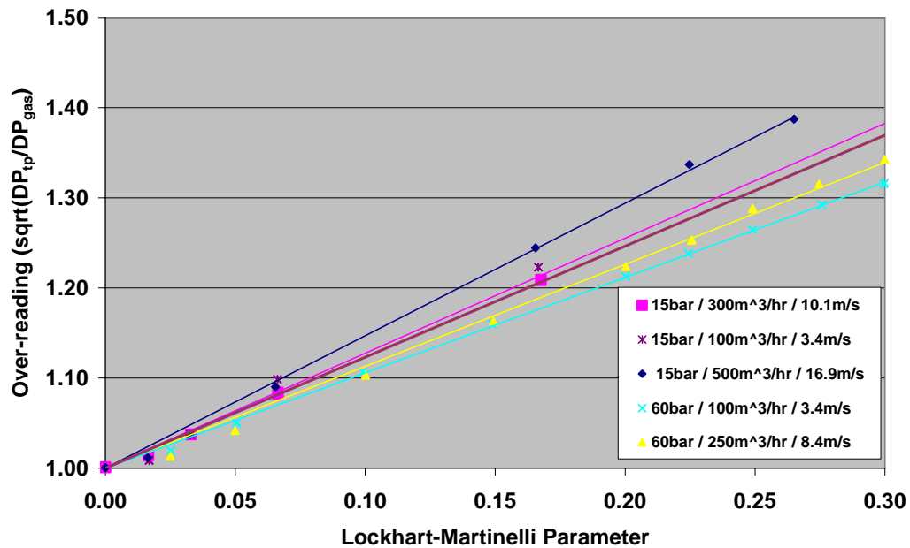
Figure 3: Relationship between Lockhart-Martinelli parameter and overreading for a typical V-Cone
