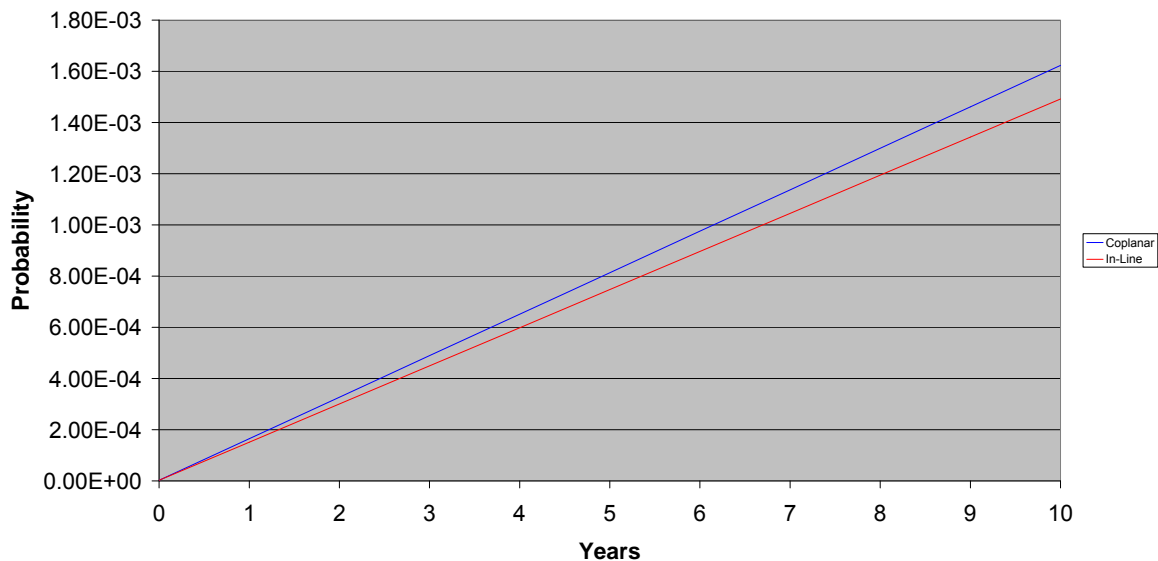
Figure 1 PFD AVG (t) 3051C / 3051T / 3051L pressure transmitter, Software Revision 7.0 and above
