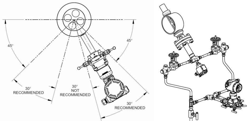
Figure 1: Traditional Steam DP Flowmeter Installation.
