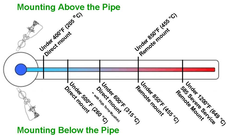
Figure 2: Annubar Steam Upper Temperature Limits.
