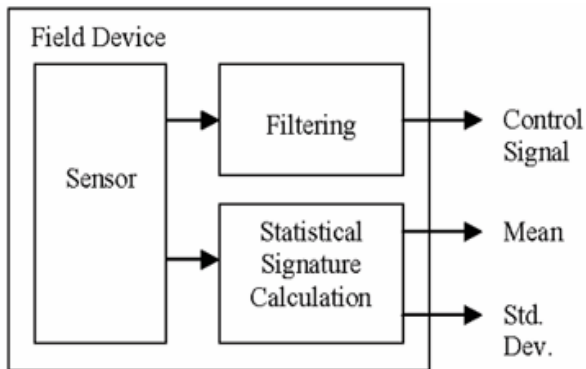
FIGURE 1. Field Device Providing both Control Signal and Advanced Diagnostics Data
