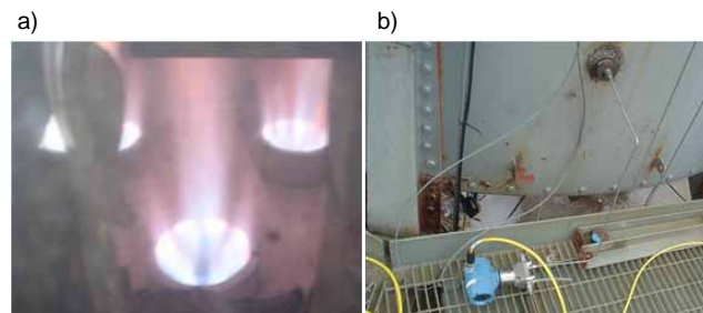
FIGURE 4. a.) Furnace Burners Seen through the Viewport b.) Pressure Transmitter Connected to the Furnace Measuring Draft Pressure
