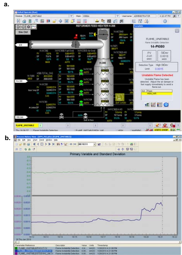
FIGURE 7. Furnace Flame Instability Detection in a Control System: a.) Operator Interface showing Flame Instability Alert; b.) Trending Advanced Diagnostics Data in Process Historian
