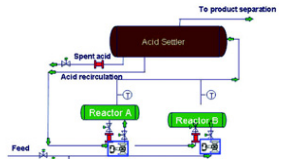
Typical diagram of the alkylation process
