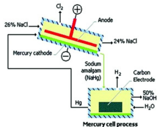
Schematic of Mercury Cell Electrolysis Process.
