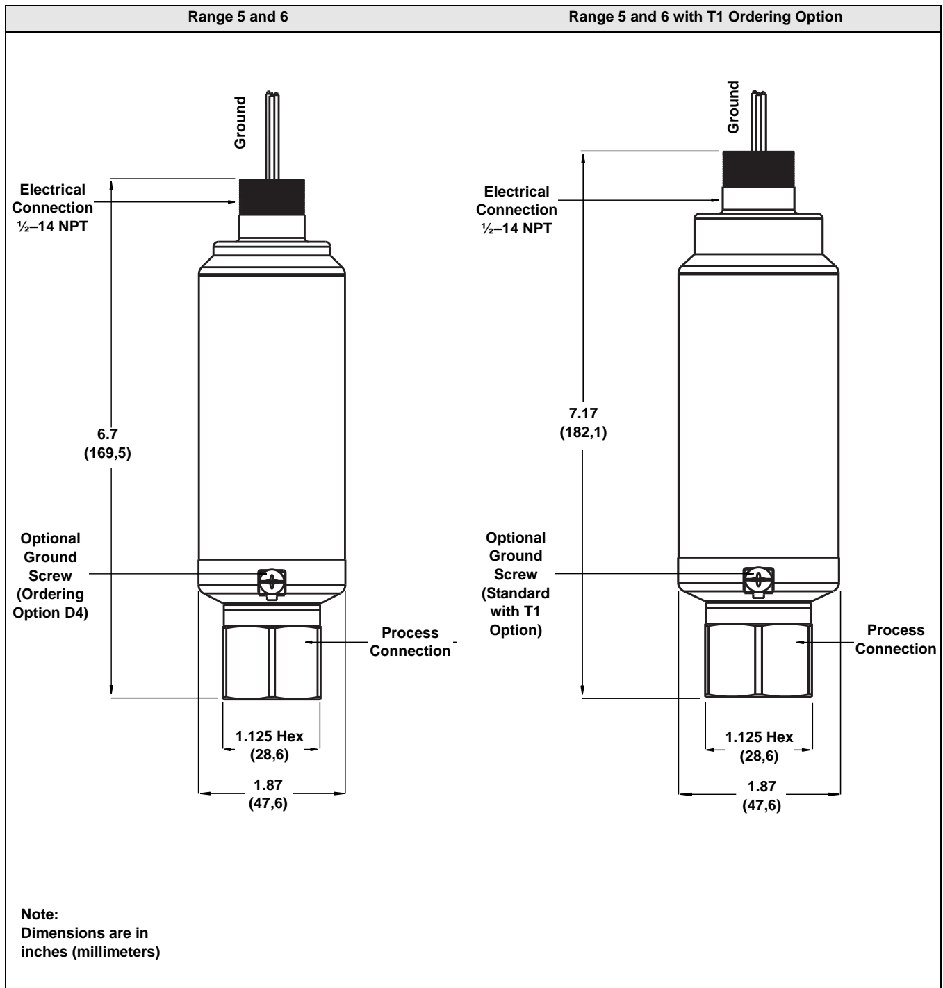
Figure 2. Dimensional Drawings for the Rosemount 4600 Oil & Gas Panel Pressure Transmitter
