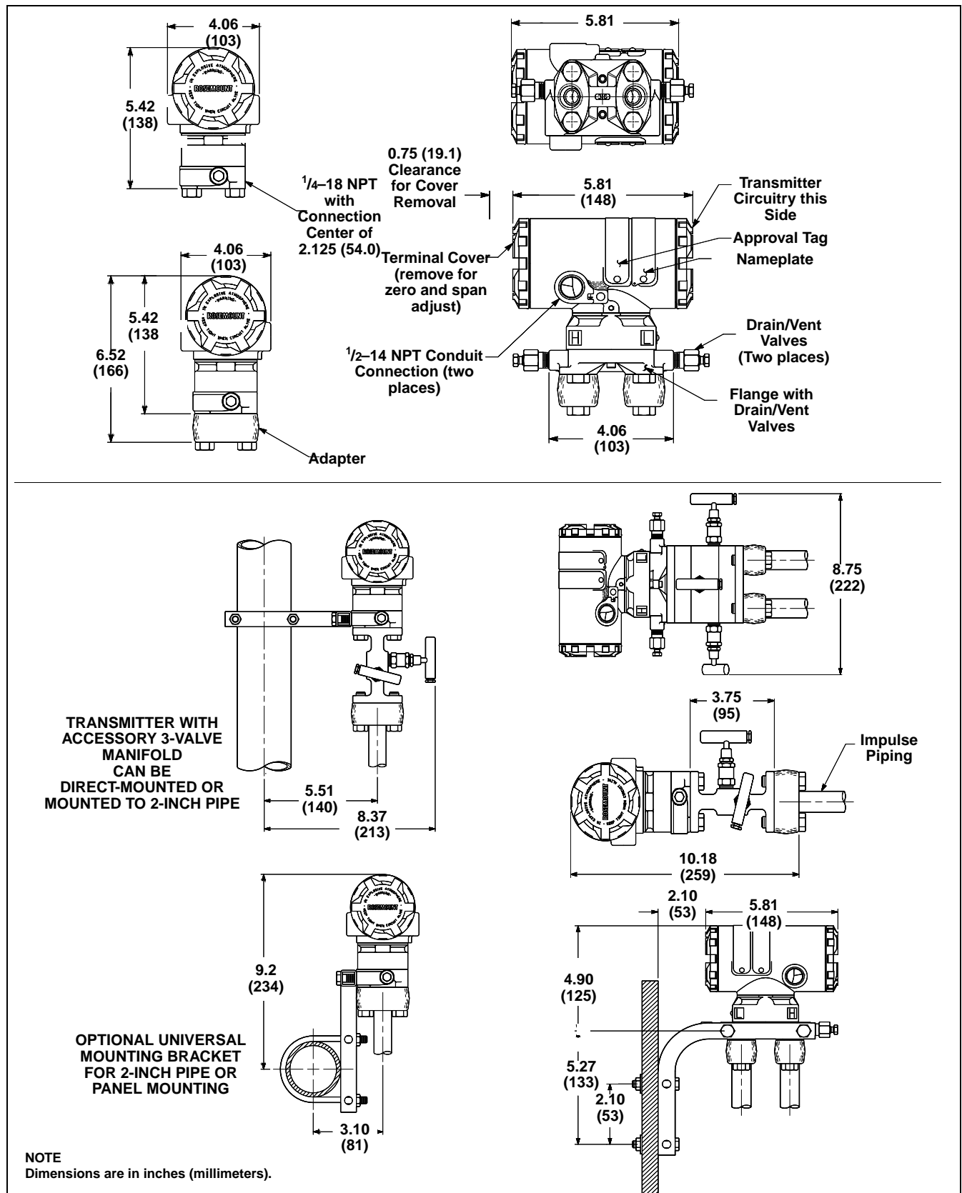
Figure 6-1. Dimensional Drawing and Mounting Configurations.
