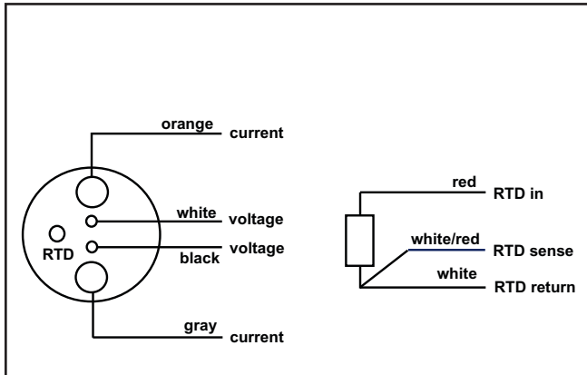
Figure 1. Wire color and functions. Current is injected through the gray and orange wires. Voltage is measured across the white and black wires.
