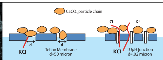
Comparison of reference junction types
