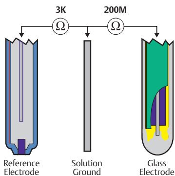
pH Sensor Components
