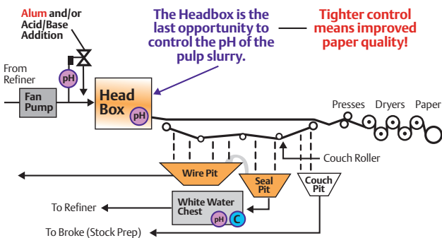
Paper Machine Overview
