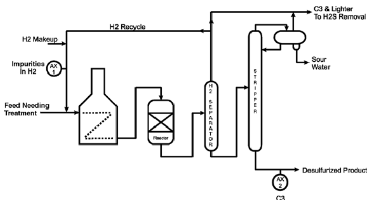
Figure 1 - Flow Diagram of a Typical Hydrotreater Unit in a Refinery
