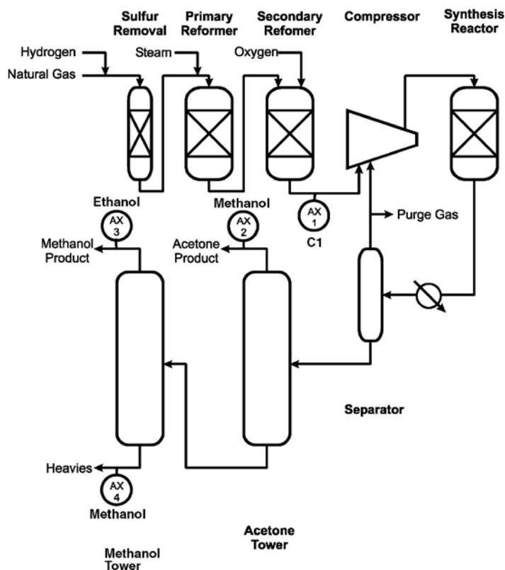
Figure 1 - Flow Diagram of a Typical Methanol Plant
