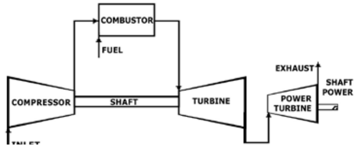
Figure 1 - Flow Diagram of a Typical Combustion Turbine
