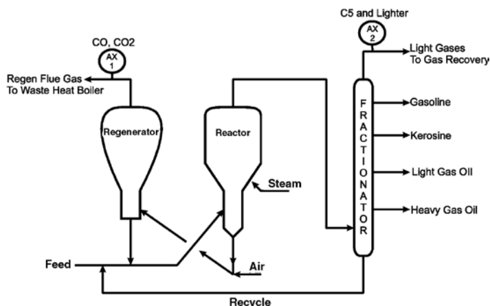
Figure 1 - Flow Diagram of a Typical Fluid Catalytic Cracking Unit
