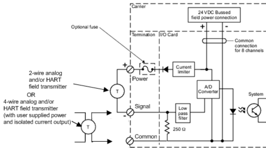
Simplified circuit and connection diagram for HART AI-card, 8 channel, 4 to 20 mA
