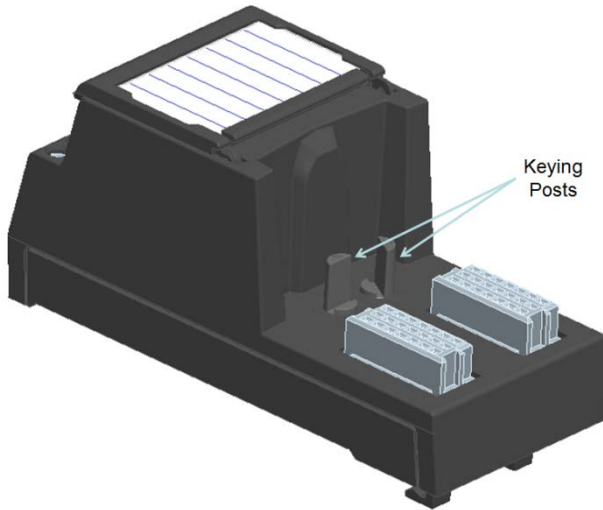
8 channel standard Terminal block
