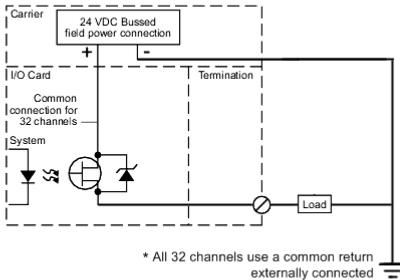
Simplified circuit and connection diagram for High Density DO card, 32 channel, 24 VDC, High Side
