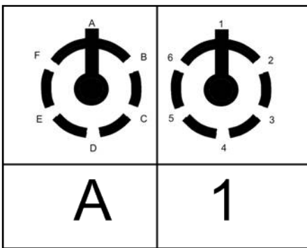
Keying position for HART AI, 4-20 mA, 8 channel
