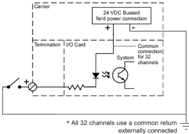
Simplified circuit and connection diagram for High Density DI card, 32 channel, 24 VDC, Dry contact
