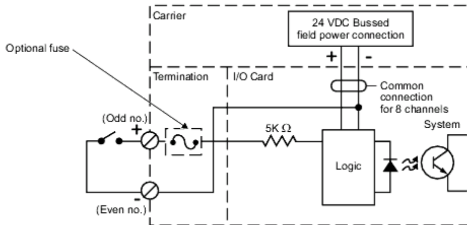
Simplified circuit and connection diagram for DI card, 8 channel, 24 VDC, NAMUR
