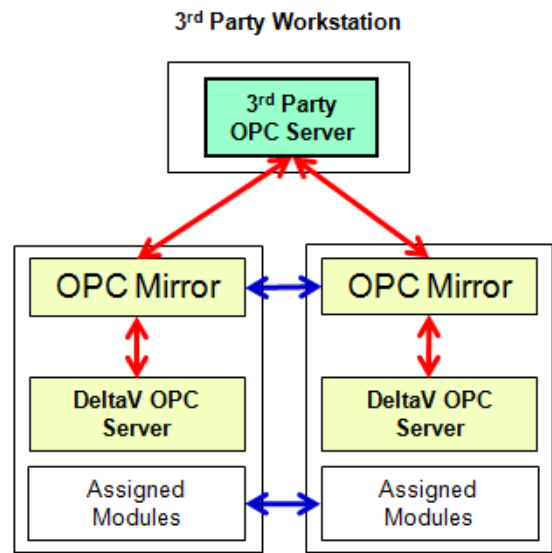
Application Station Pair (Active/Standby)
