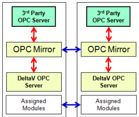
Application Station Pair (Active/Standby)
