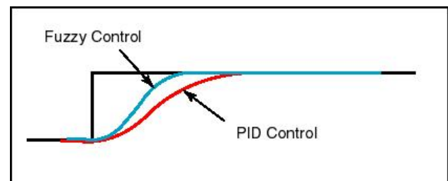
PID tuned for no overshoot.
