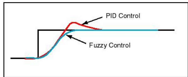
PID tuned with overshoot allowed.
