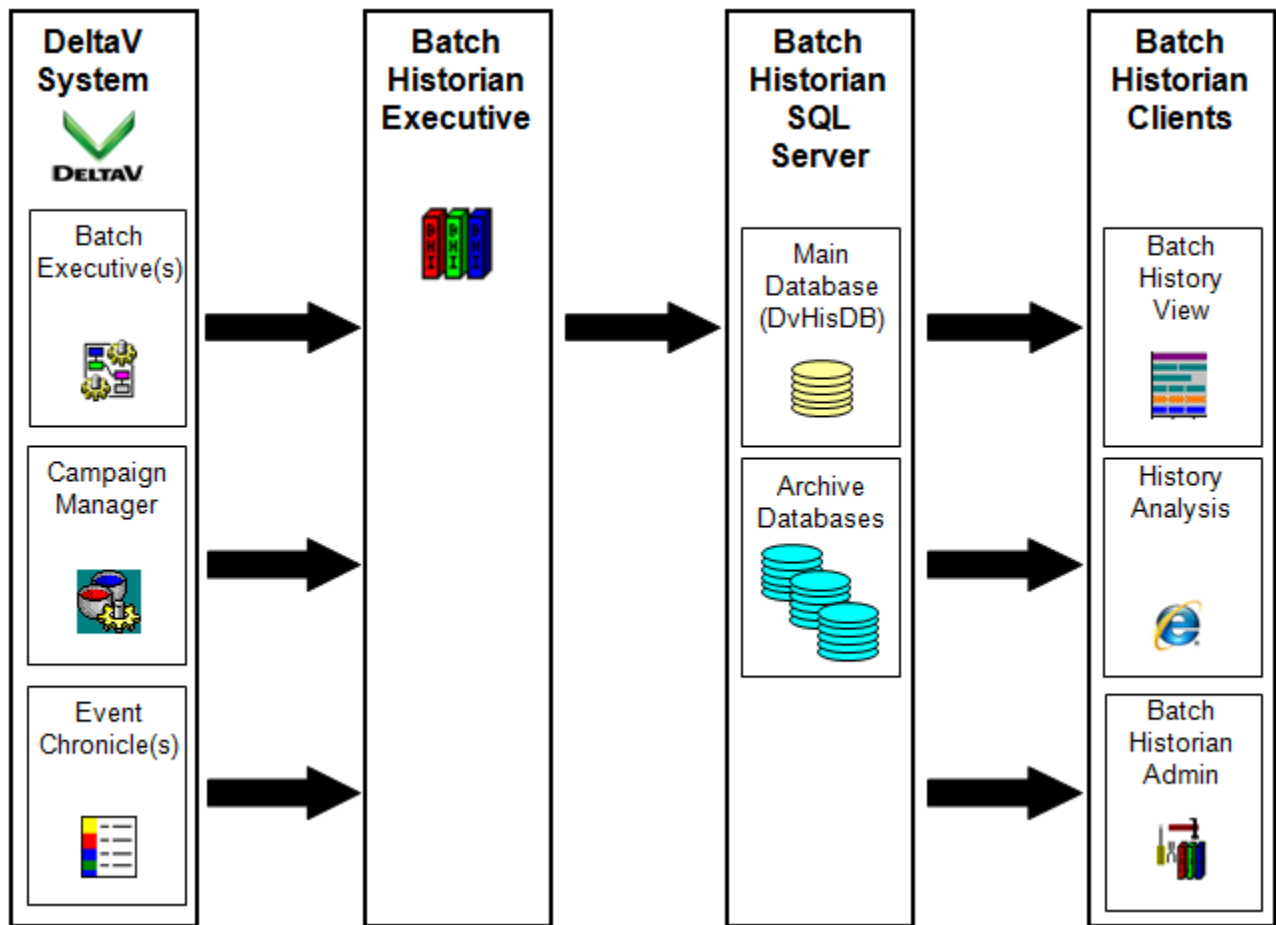
Information flow in the Batch Historian.
