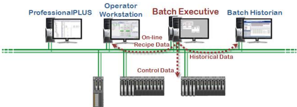
The Batch Executive processes and serves data to the DeltaV Batch application suite.
