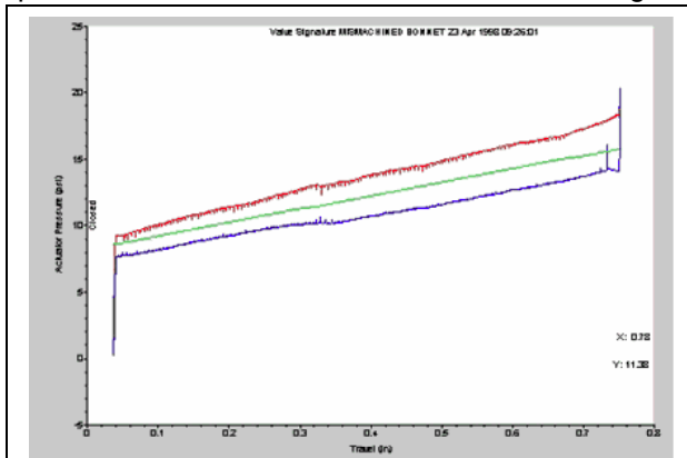
Valve signature diagnostics reveal conditions that if left undetected will increase process variability.
