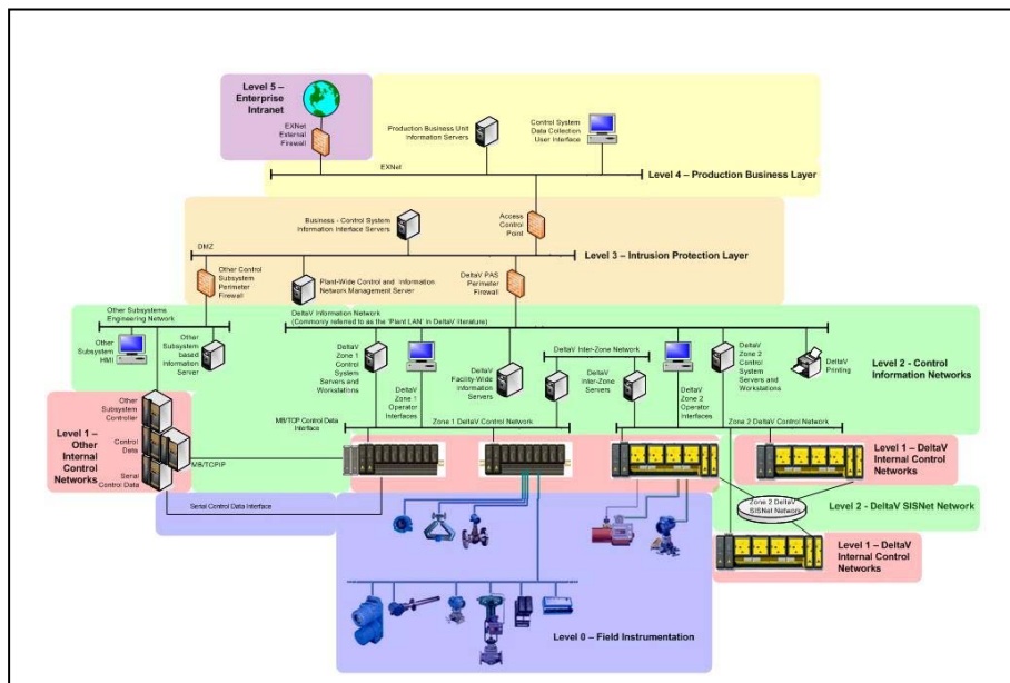
Figure 1: Typical ICSS Architecture
