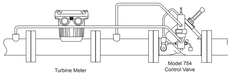
Figure 7 - Model 754 with turbine meter.
