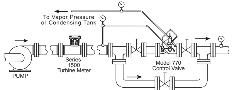
Figure 12 - The Model 770 controls differential pressure (LPG, NH 3 ).
