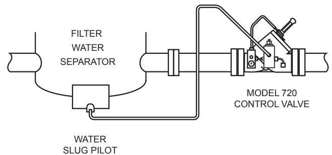
Figure 3 - Model 720 used with filter water separator tank.
