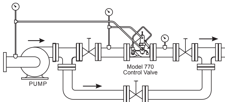
Figure 13 - The Model 770 control valve maintains minimum pump differential.
