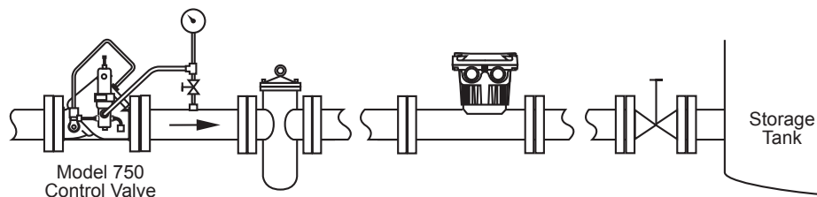
Figure 6 - In this application, the Model 750 pressure reducing valve lowers main pipeline pressure to a level that is within the acceptable rating of the metering equipment. The pressure reducing valve will control a maximum reduced pressure drop of 1,000 psi (6,995 kPa).
