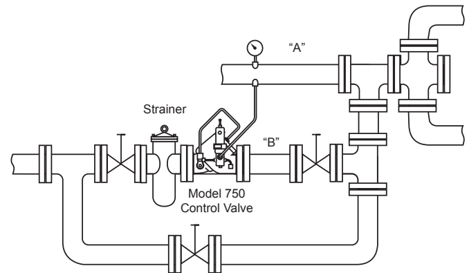
Figure 5 - Pipeline "A" normally provides all the product for distribution unless pressure drops below a required minimum. When this occurs the Model 750 installed in an auxiliary line "B" and sensed to the main line "A", opens to maintain pressure and flow until normal main line pressure is restored.
