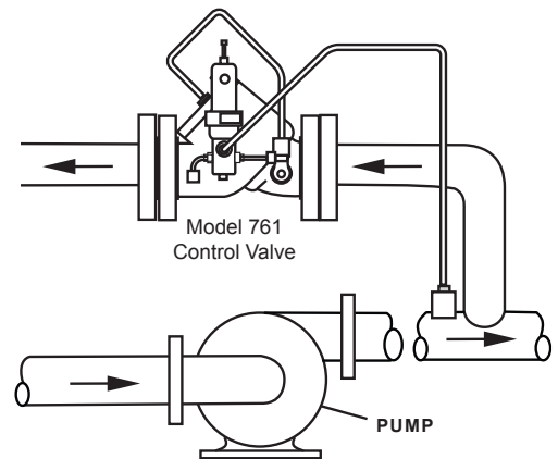
Figure 9 - The Model 761 illustrated here is applied either as a relief valve to protect the line against excessive pressure and surge or as a pump bypass valve to maintain a constant pump discharge. Flow through the valve may be piped to storage, pump suction, sump, or atmosphere.
