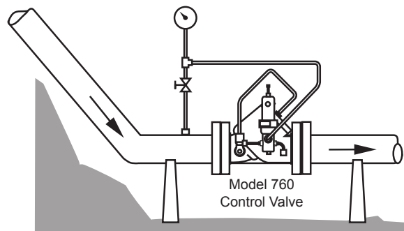
Figure 10 - The Model 760 installed in a pipeline at the bottom of an incline. The valve maintains a back pressure equal to head pressure and prevents liquid separation.
