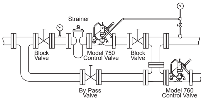
Figure 4 - This drawing illustrates the most common usage of the pressure reducing control valve. The Model 750 externally sensed to any point downstream, provides a sensitive control for regulation of pressure within \pm 2 psi (13.8 kPa). The Model 760 back pressure control valve, acting as a relief valve, protects the system if excessive pressure or surge occurs.
