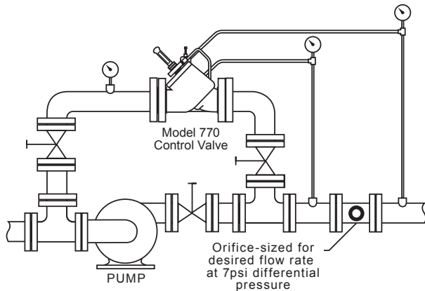
Figure 11 - The Model 770 control valve bypasses rate of flow control.
