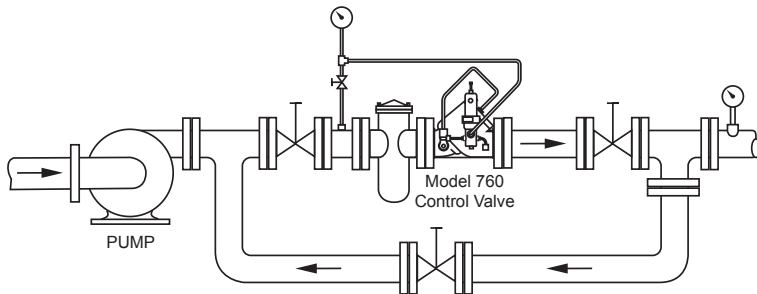
Figure 8 - The Model 760 is used to maintain constant pressure at the pump discharge. The valve opens when a predetermined pressure is reached, allowing flow to start, then it regulates back pressure on the pump within \pm 2 psi (13.8 kPa).
