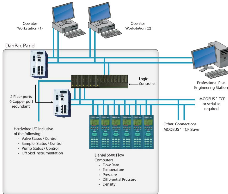
DanPac System Architecture with Two Workstations (Source: Daniel Measurement and Control)
