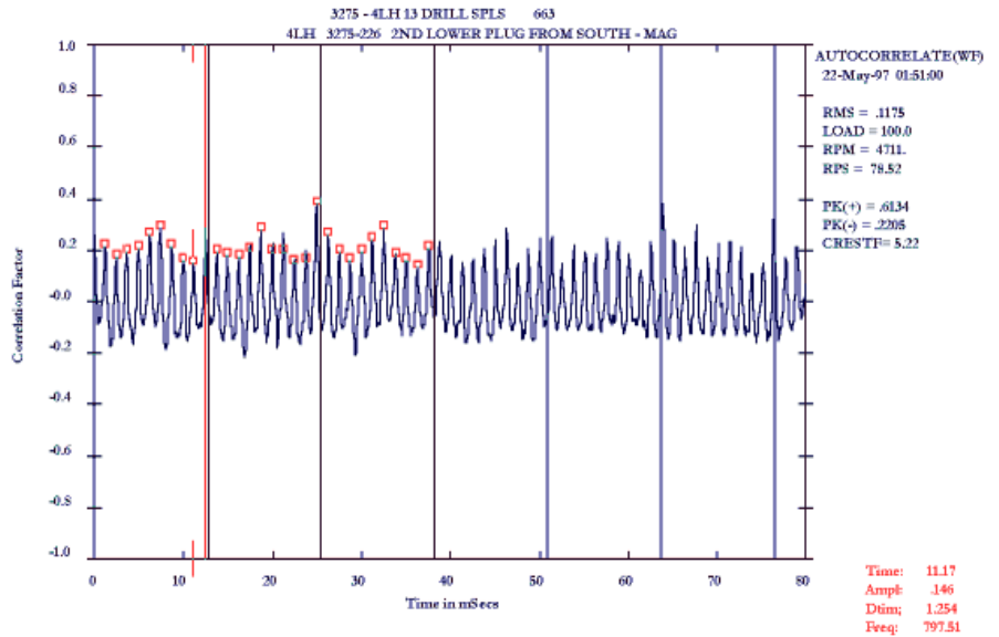
Figure 10. Autocorrelation coefficient from PeakVue time waveform acquired on the spindle of Figure 9.
