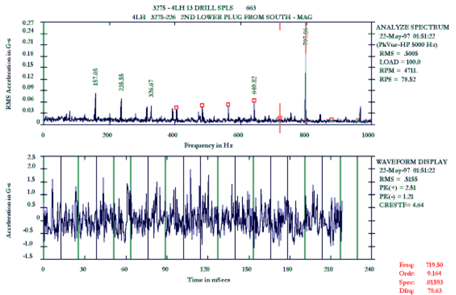
Figure 9. PeakVue spectra and time waveform from a spindle on a 13 multi-drill head spindle.
