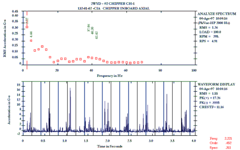
Figure 12. PeakVue Spectra and time waveform from inboard axial on chipper.
