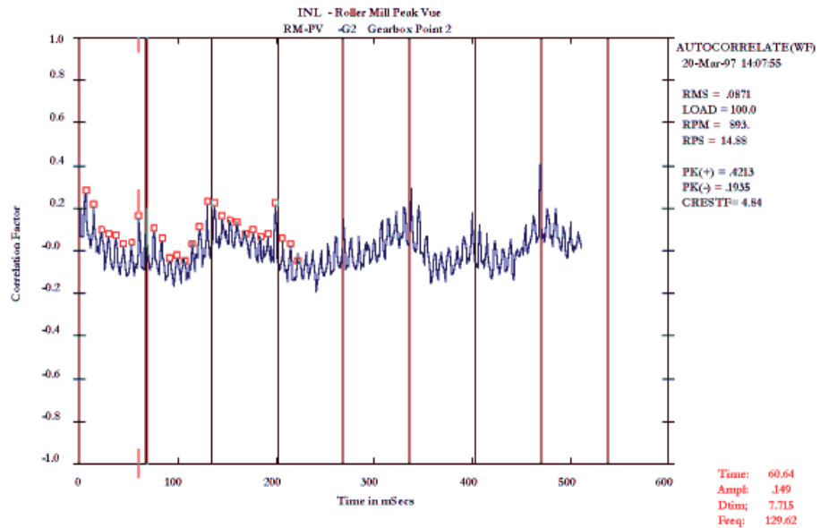
Figure 8. Autocorrelation coefficient from PeakVue time waveform of Figure 7.
