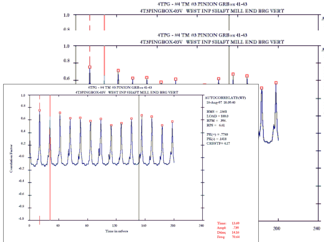
Figure 2: Autocorrelation coefficient from PeakVue time waveform in Fig 1
