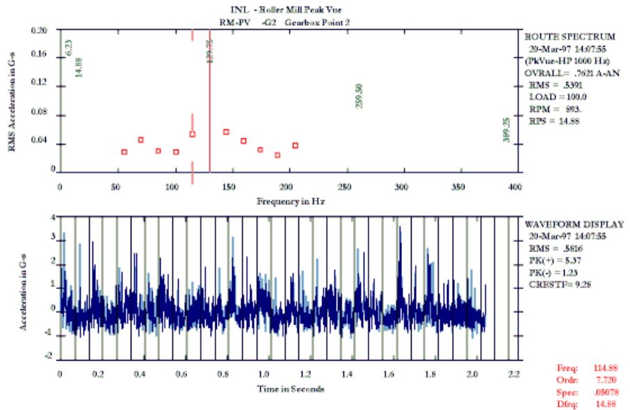
Figure 7. PeakVue spectra and time waveform from inlet of crusher gear box.
