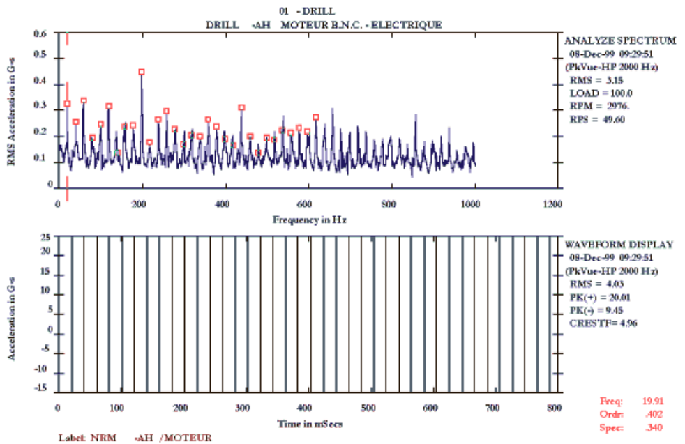
Figure 20. PeakVue Spectra and Time Waveform on the outboard bearing of the male rotor and simple stage compressor.
