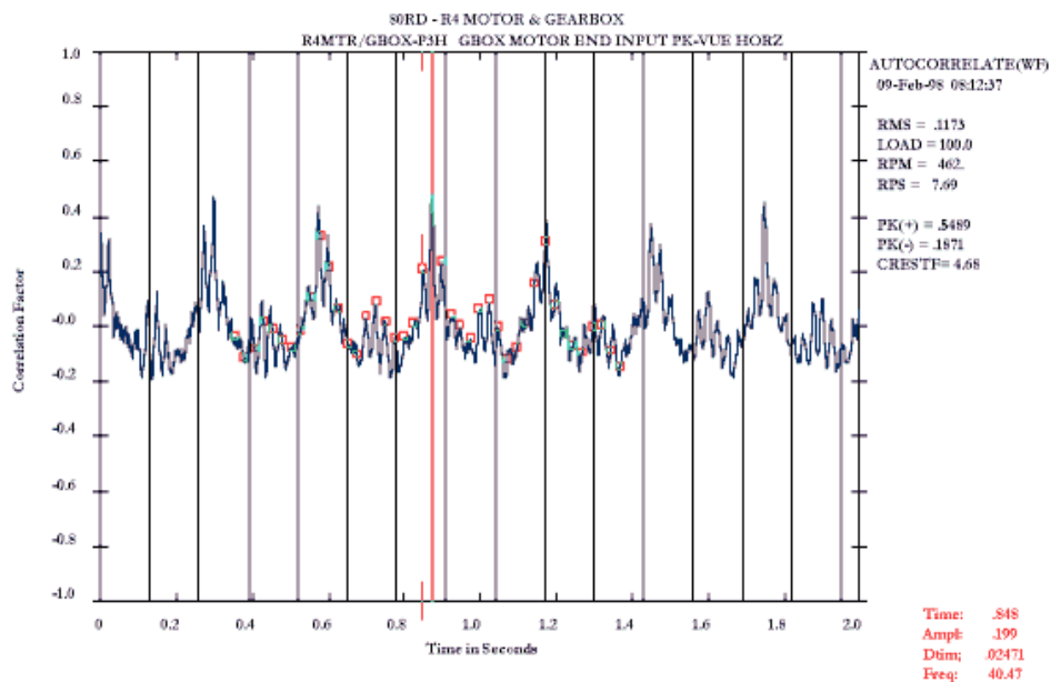
Figure 15. Autocorrelation coefficient from PeakVue time waveform of Figure 14.
