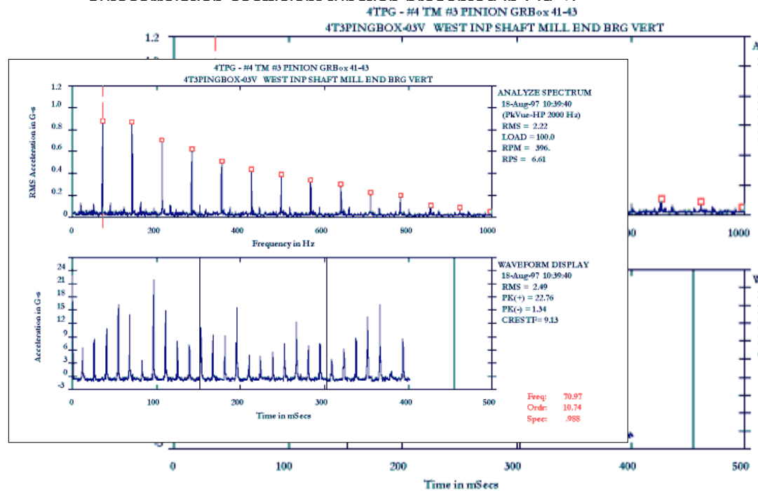
Figure 1: PeakVue Spectra and time waveform from input shaft of pinion stand gearbox
