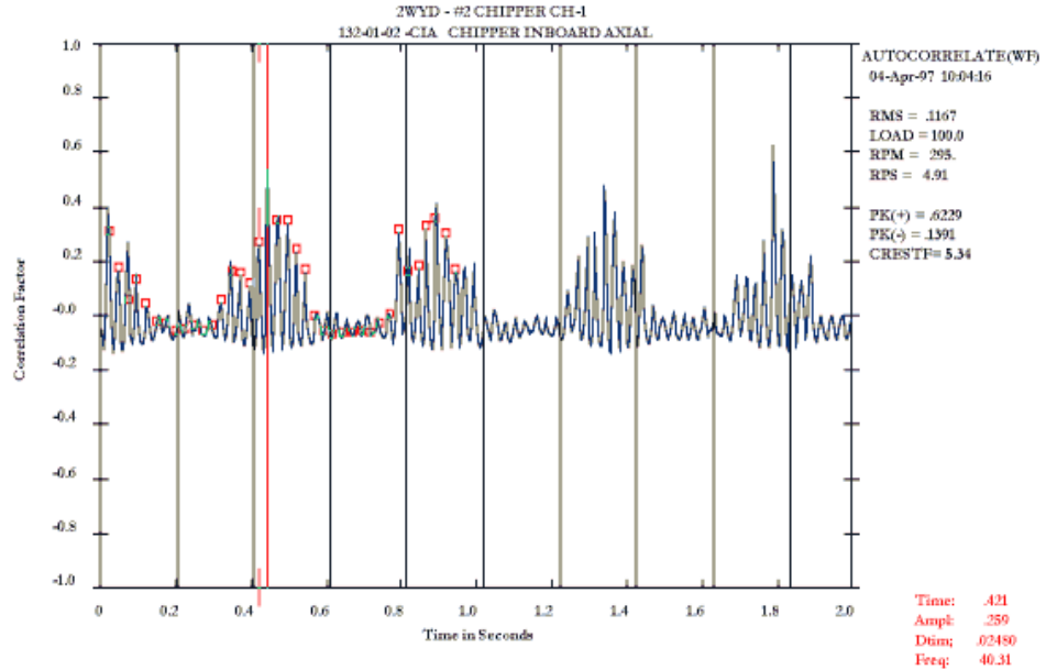
Figure 13. Autocorrelation coefficient from PeakVue time waveform of Figure 12.
