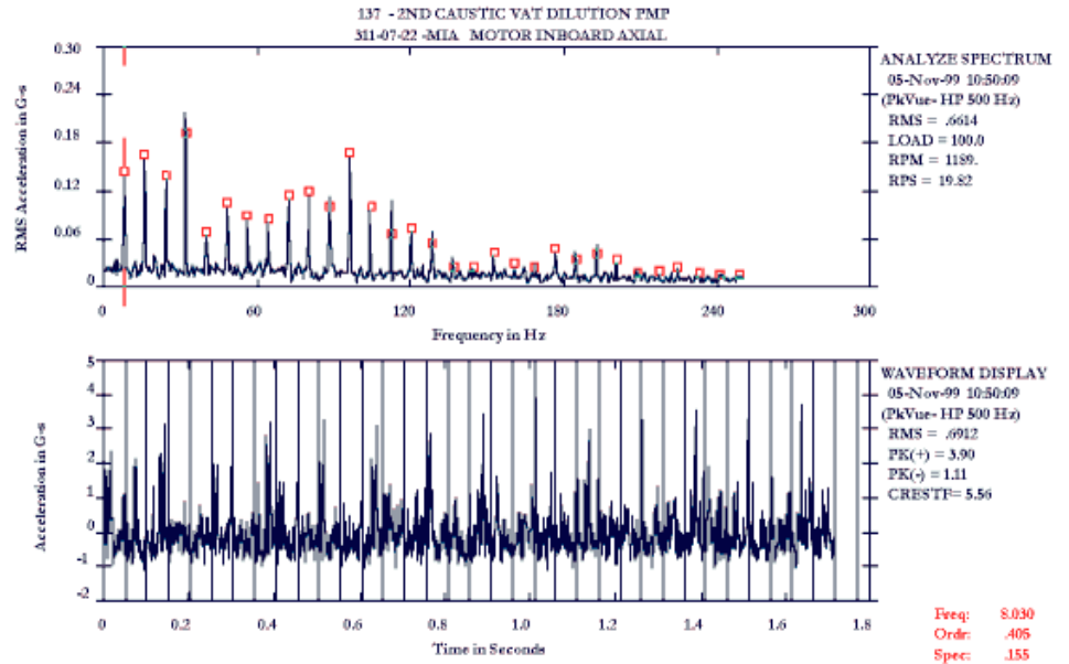
Figure 17. PeakVue spectra and time waveform from Motor (Inboard Axial) driving direct coupled centrifugal pump.
