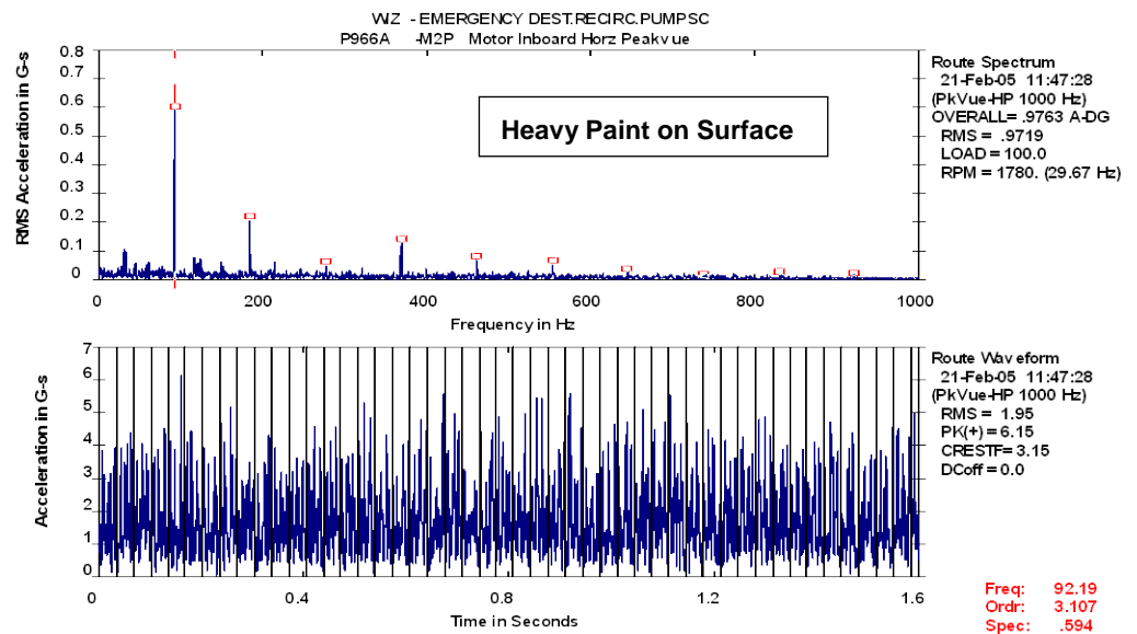
Figure 13. PeakVue Data from Inboard Motor Bearing Showing BPFO Fault in the Early Alert Stage (6.2 g's Peak).
