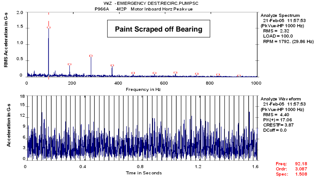
Figure 14. PeakVue Data from Same Point Presented in Figure 13, 10 Minutes Later Following Removing Paint Where Sensor was Located. g-level Increased from 6.2 g's (Early Alert) to 17 g's (Serious Fault).
