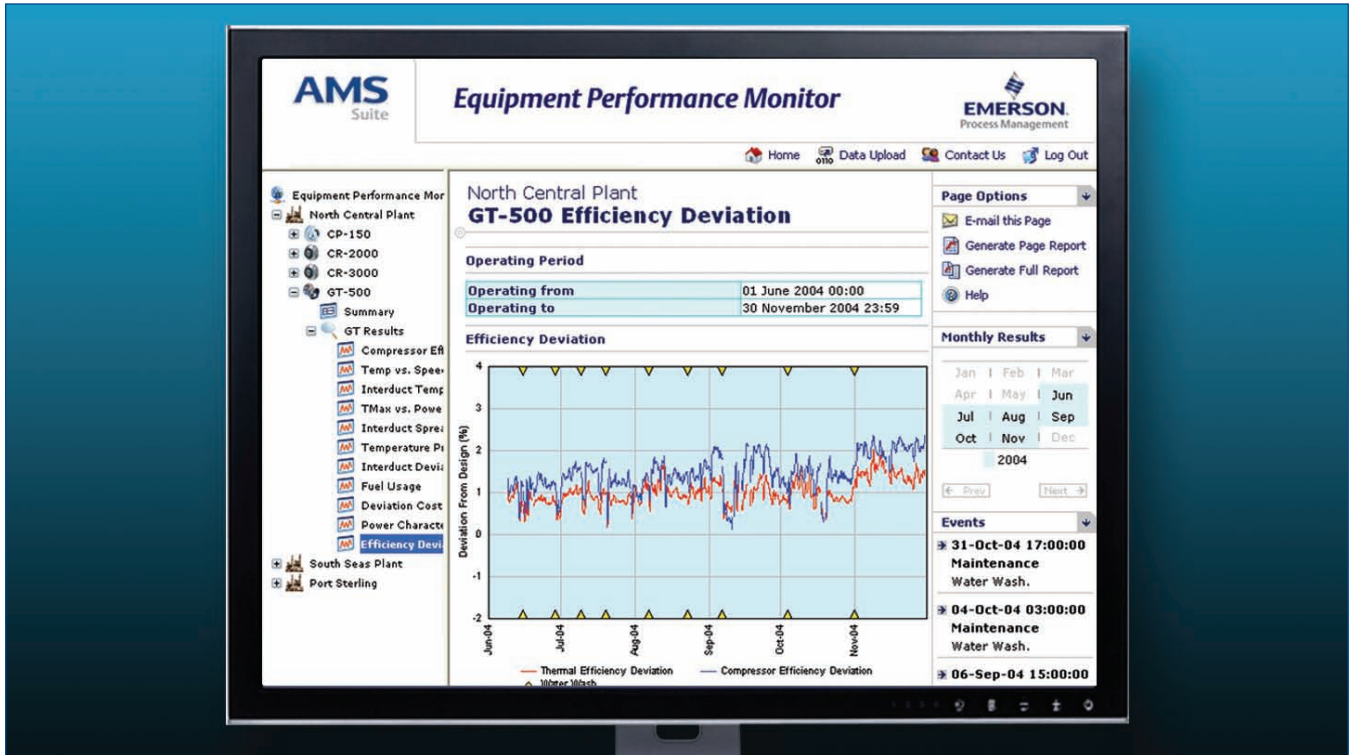
Difference between actual and design gas turbine thermal efficiency and compressor efficiency.
