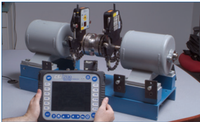
CSI 8225 Laser Heads
