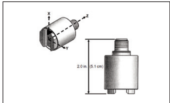
Emerson's patented triaxial sensor with integral magnet
