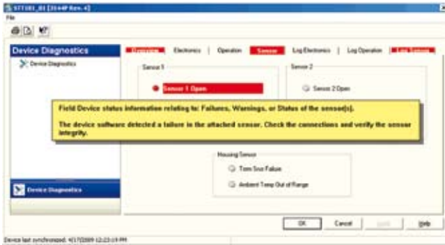
SIS transmitter diagnostics displayed based on EDDL, including manufacturer's help text.
